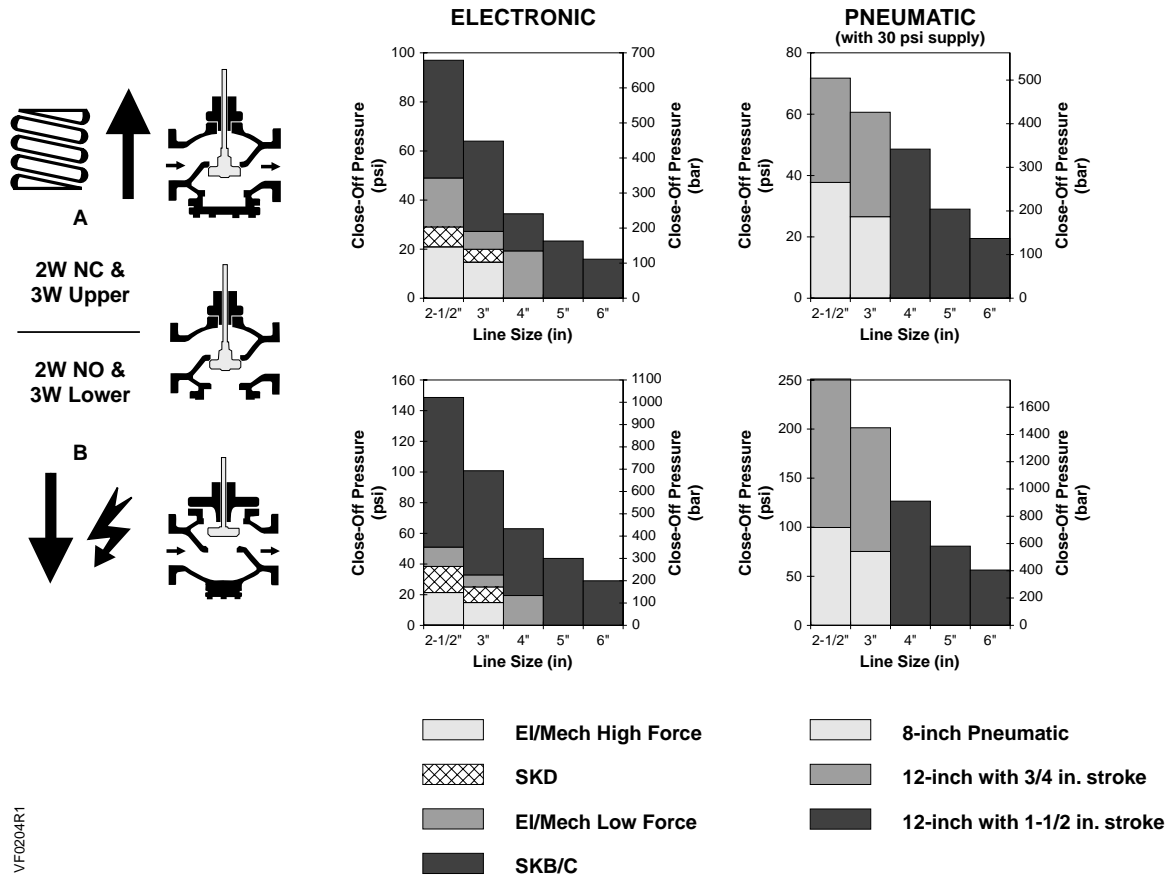
Figure 3. Close-off Pressures.
